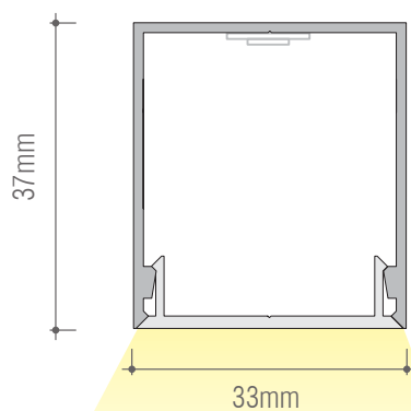
Snap P2 LED
