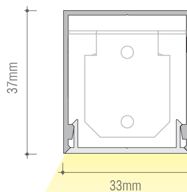
Snap P2 T5
